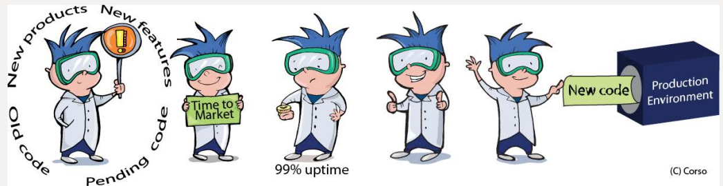
Figure 54: Continuous delivery
