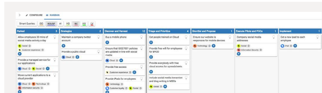
Figure 12: Kanban board
